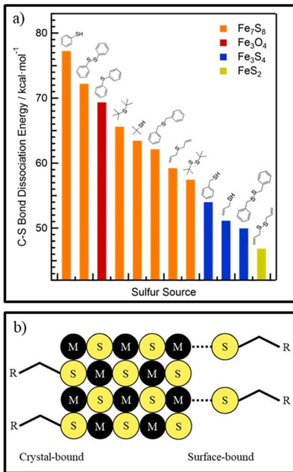
Fig. 5 (a) Reactivity of different sulfur precursors vs. the carbon–sulfur dissociation energy and their products in iron sulfide synthesis. Adapted with permission from ref. 89. Copyright 2017 American Chemistry Society. (b) Schematic picture of crystal-bound and surface-bound thiols. Adapted with permission from ref. 90. Copyright 2014 American Chemistry Society.
