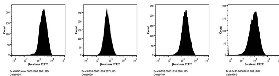
Fig. 14 Expression studies of the β-catenin protein towards HepG2 cells.
