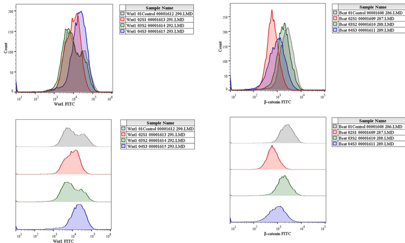
Fig. 15 Expression studies of the β-catenin protein towards HepG2 cells.
