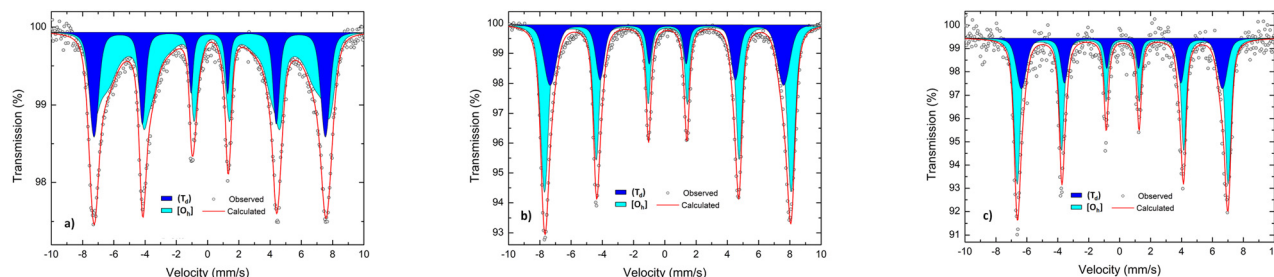
Fig. 4 The room-temperature ^{57}\text{Fe} Mössbauer spectra of (a) HEOFe, (b) LiHEOFef, and (c) LiHEOFefCl. The dark blue and light blue spectra correspond to tetrahedrally ( T_d ) and octahedrally ( O_h ) coordinated iron cations, respectively.
