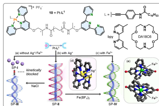
Fig. 9 Structure of 10 and the secondary mechanism of SPs from 10 in the (a) absence and (b and c) presence of secondary metal ions (Ag + and Fe 2+ ) and (d and e) partial chemical structures of the 10 complexes with (d) Ag + and (e) Fe 2+ ions obtained by DFT calculation. Reproduced from ref. 52 with permission from Royal Society of Chemistry, copyright 2024.
