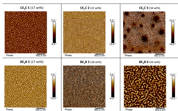
Fig. 8 AFM phase image of triblock copolymer with PCaMA (CE 3 C 5, CE 1 C 2 and CE 1 C 3) or PBetuma (BE 3 B 5, BE 1 B 3 and BE 3 B 6) as external blocks. Corresponding topography images in ESI, Fig. S19.†
