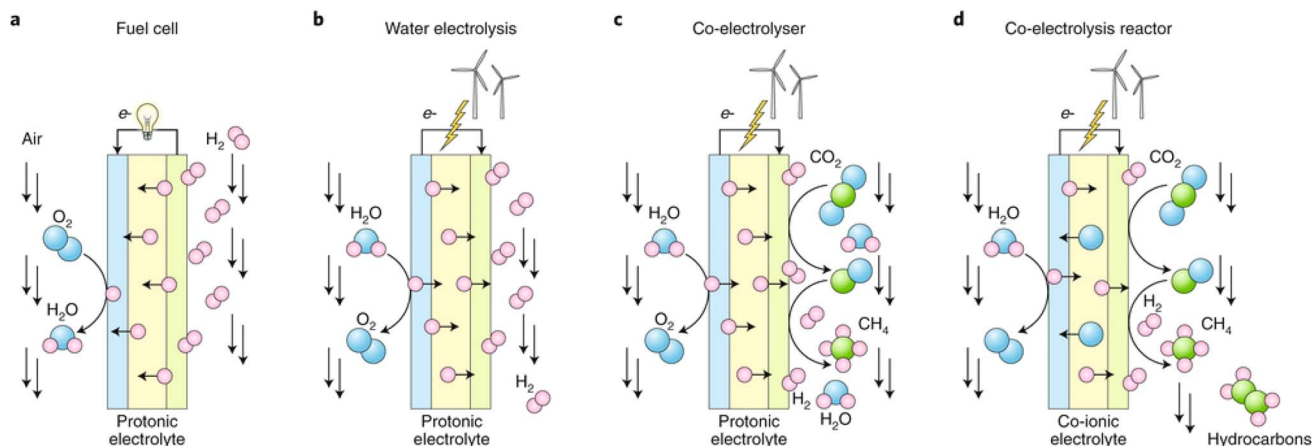
Fig. 15 The different working principles of H-SEMRs: (a) fuel cell, (b) electrolyzer cell, (c) \text{CO}_2/\text{H}_2\text{O} co-electrolysis, and (d) co-electrolysis reactor based on co-ionic conductor. 66,265 Reproduced with permission.
