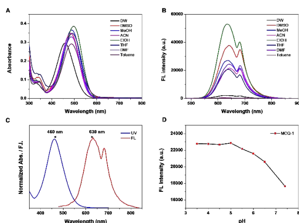
Figure 1 (A) UV–vis absorption and (B) fluorescence spectra of MCQ-1 (10 \mu M) in different solvents; \lambda_{\text{ex}} = 460 nm. (C) Normalized absorption and emission spectra of MCQ-1 (10 \mu M) in ACN/PBS solution (5:95, v/v). (D) Fluorescence spectra of MCQ-1 (10 \mu M) at different pH values; the inset shows the corresponding intensities at 630 nm.
