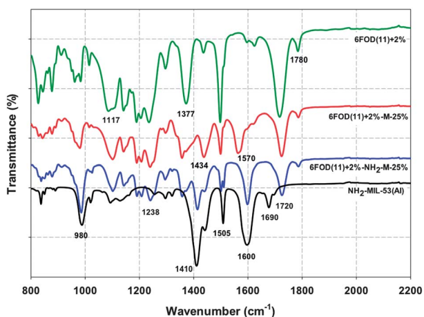
Fig. 8 ATR-FTIR spectra between 800 and 2200 \text{cm}^{-1} for \text{NH}_2 -MIL-53(Al), 6FOD(11) + 2% and their MMMs (all spectra are shifted upward by 2.5, 5.0, and 7.5%, respectively, except \text{NH}_2 -MIL-53(Al)).
