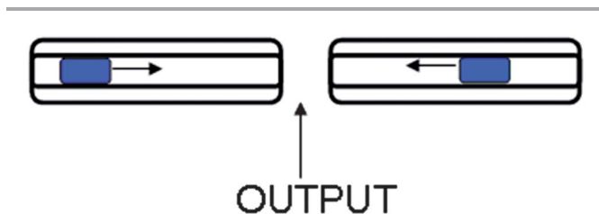
Fig. 16 Schematic representation of two blue waves propagating through two capillary tubes and ending in a middle compartment where they interact.
