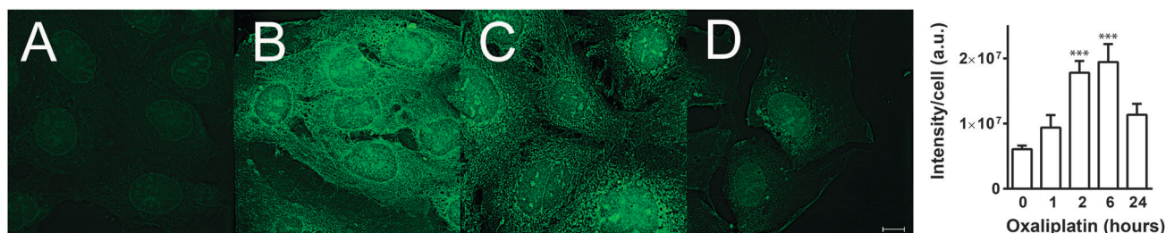
Fig. 2 Deconvoluted fluorescence images of Caco-2 cells treated with FDCPt1 (20 \mu M) for 30 min alone (A) or with FDCPt1 after incubation with oxaliplatin (20 \mu M) for 1 (B), 6 (C) or 24 h (D). Scale bar represents 10 \mu m.
