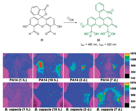
Fig. 26 Top: fluorescein dialdehyde chemodosimeter 31 for ^-CN . Bottom: in vivo images of ^-CN in the lungs after various incubation times after infection with PA and Bcc . Colour images were reconstructed from inverted fluorescence images. Image reproduced with permission. 172
