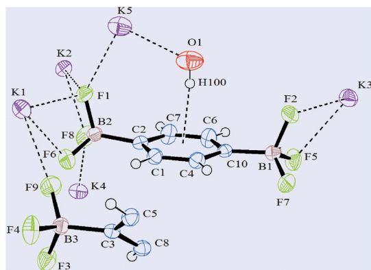
Fig. 1 ORTEP-plot of the asymmetric unit of the title compound 2 with ellipsoids plotted at the 50% probability level. Short K...F, K...O contacts and OH...π interactions are drawn as dashed lines. Colour codes in the electronic version of the paper: carbon (blue), boron (light brown), fluorine (green), potassium (violet) and oxygen (red). Hydrogen atoms are also drawn as small spheres.
