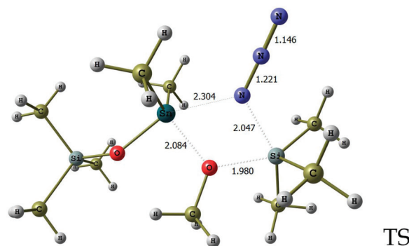
Scheme 6 Simplified computed reaction for the evaluation of the tin to silicon exchange leading to 48.
