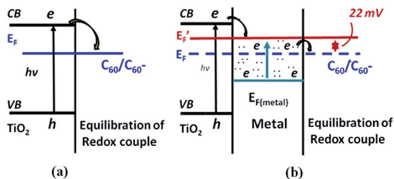
Fig. 2 Charge distribution between TiO 2 and gold nanoparticles leading to equilibration with the C 60 /C 60 - redox couple (a) in the absence and (b) in the presence of metal nanoparticles. E F and E F ' refer to the Fermi levels of TiO 2 before and after attaining equilibrium, respectively. Figure reprinted with permission from ref. 50.
