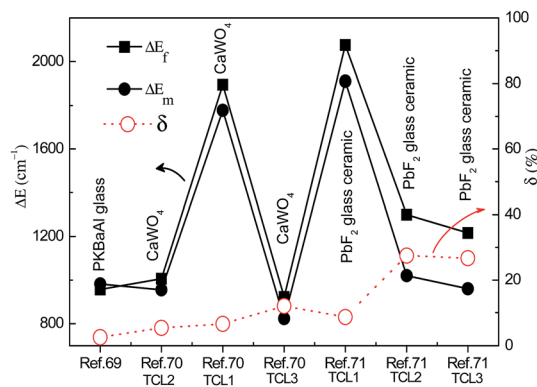
Fig. 14 Host dependent \Delta E_f and \Delta E_m between the TCL of \text{Nd}^{3+} ions, and the corresponding \delta values.
