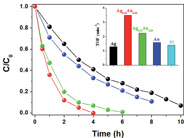
Fig. 3 Catalytic reduction of 4-NP by \text{Ag@CeO}_2 (black), \text{Ag}_{0.64}\text{Au}_{0.36}\text{@CeO}_2 (red), \text{Ag}_{0.41}\text{Au}_{0.59}\text{@CeO}_2 (green) and \text{Au@CeO}_2 (blue). Inset: calculated TOF compared with \text{Pt@CeO}_2 . 7
