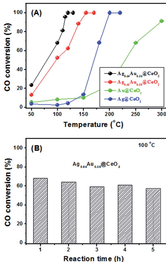
Fig. 4 (A) CO conversion curves of \text{Ag@CeO}_2 , \text{Ag}_{0.64}\text{Au}_{0.36}\text{@CeO}_2 , \text{Ag}_{0.41}\text{Au}_{0.59}\text{@CeO}_2 and \text{Au@CeO}_2 ; (B) cycling test of \text{Ag}_{0.64}\text{Au}_{0.36}\text{@CeO}_2 at 100 \text{ }^\circ\text{C} for 5 h.
