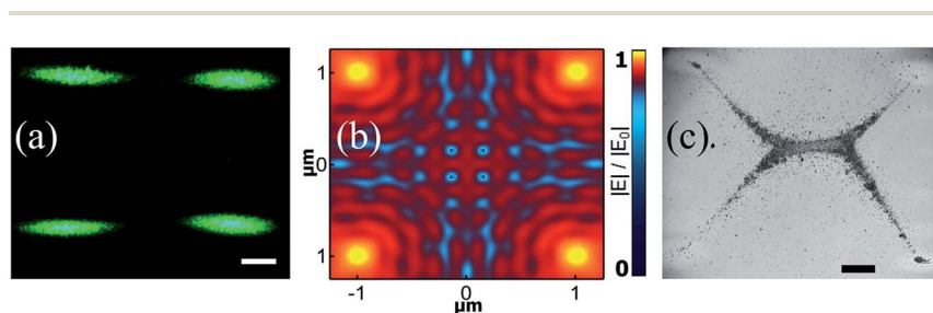
Fig. 4 Plasmofluidic assembly of nanoparticles using quadruple-trap configuration. (a) Optical dark-field image of the four, evanescently-excited 532 nm laser spots on a gold film (50 nm thick) optically coupled to the Dove prism. Scale bar is 200 \mu\text{m} . (b) Simulated electric near-field distribution of the four laser spots at the gold–water interface. The geometry of the simulation was identical to the experimental configuration. Plasmonic interference patterns can be clearly observed. (c) Optical bright-field image of plasmofluidic assembly of Ag nanoparticles at gold film–water interface due to excitation shown in (a). Scale bar is 200 \mu\text{m} . The nanoparticle densities at the corners of the geometry are different due to small variance in the laser powers.
