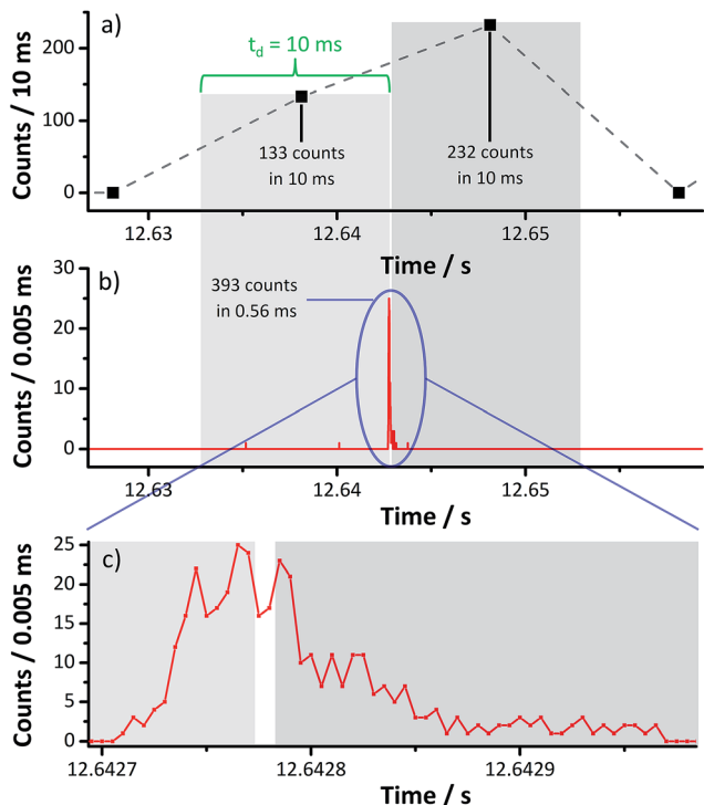
Fig. 5 Transient signal of 30 nm AuNPs ( C_{\text{NP}} = 2.5 \times 10^5 NP mL -1 ) simultaneously acquired with ICP-MS software (a) and the home-built DAQ (b) for 30 ms. A potential problem in single particle ICP-MS due to split-particle events was observed when a particle-related ion cloud occurred exactly between two adjacent dwell time intervals (grey rectangles indicate 10 ms dwell time intervals used in the ICP-MS software). Zoom-in in (c) shows the temporal profile of the particle's ion cloud with a duration of 290 \mu s.
