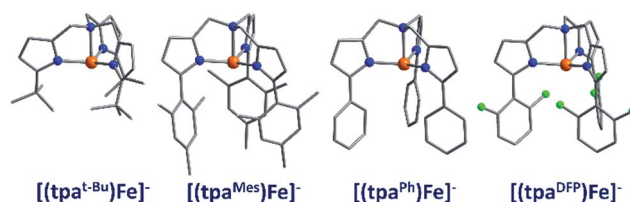
Fig. 9 Molecular structures of four coordinate trigonal pyramidal Fe(II) complexes of the form [(\text{tpa}^{\text{R}})\text{Fe}]^- . Colour code: orange (Fe), green (N), blue (C), grey (C). Hydrogen atoms omitted for clarity.
