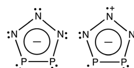
Scheme 1 Schematic depiction of P_2N_3^- and the lowest electronic state ( ^2A_1 ) of P_2N_3^{\cdot-} .
