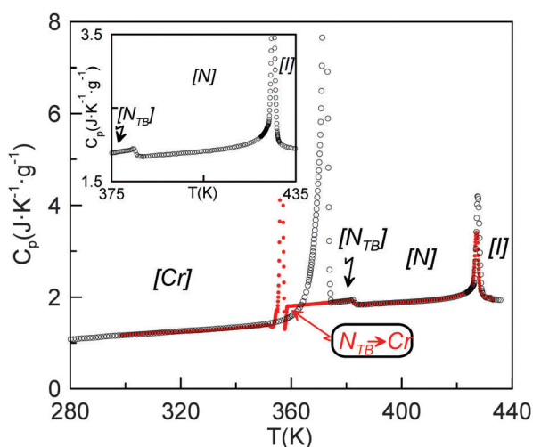
Fig. 3 Temperature dependence of the heat capacity of CB6OCB measured with an underlying heating or cooling rate of 1 \text{ K min}^{-1} . Black and red symbols correspond to heating and cooling experiments, respectively. The top-left inset provides a magnified view of the N_{TB} -N and the N-I phase transitions on heating.
