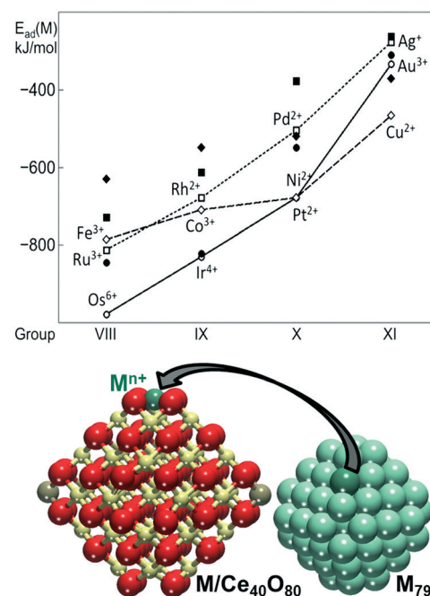
Fig. 8 Adsorption energies of atomically dispersed 3d (diamonds), 4d (squares), and 5d (circles) metals (M) on the {100} facet of the Ce 40 O 80 nanoparticle (empty symbols, connected for guiding the eye) and binding energies of these atoms in edge positions of the M 79 NP (filled symbols). The corresponding M–Ce 40 O 80 and M 79 structures are also shown. Yellow, brown and red spheres represent Ce 4+ , Ce 3+ and O 2- ions, respectively. Adapted from ref. 82 with permission from the Royal Society of Chemistry.
