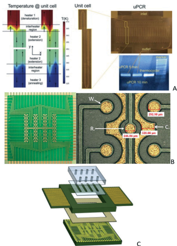
Fig. 8 A) Integrated uPCR-on-PCB (reprinted from ref. 114 with permission from Elsevier) and electrochemical biosensor array chips on a PCB, B) an electrochemically gold plated DNA detector on a PCB (from ref. 131, with permission from IOS Press) and C) a schematic representation of the sensor platform B packages with PMMA microfluidics (reprinted from ref. 132, copyright 2016, with permission from Elsevier).
