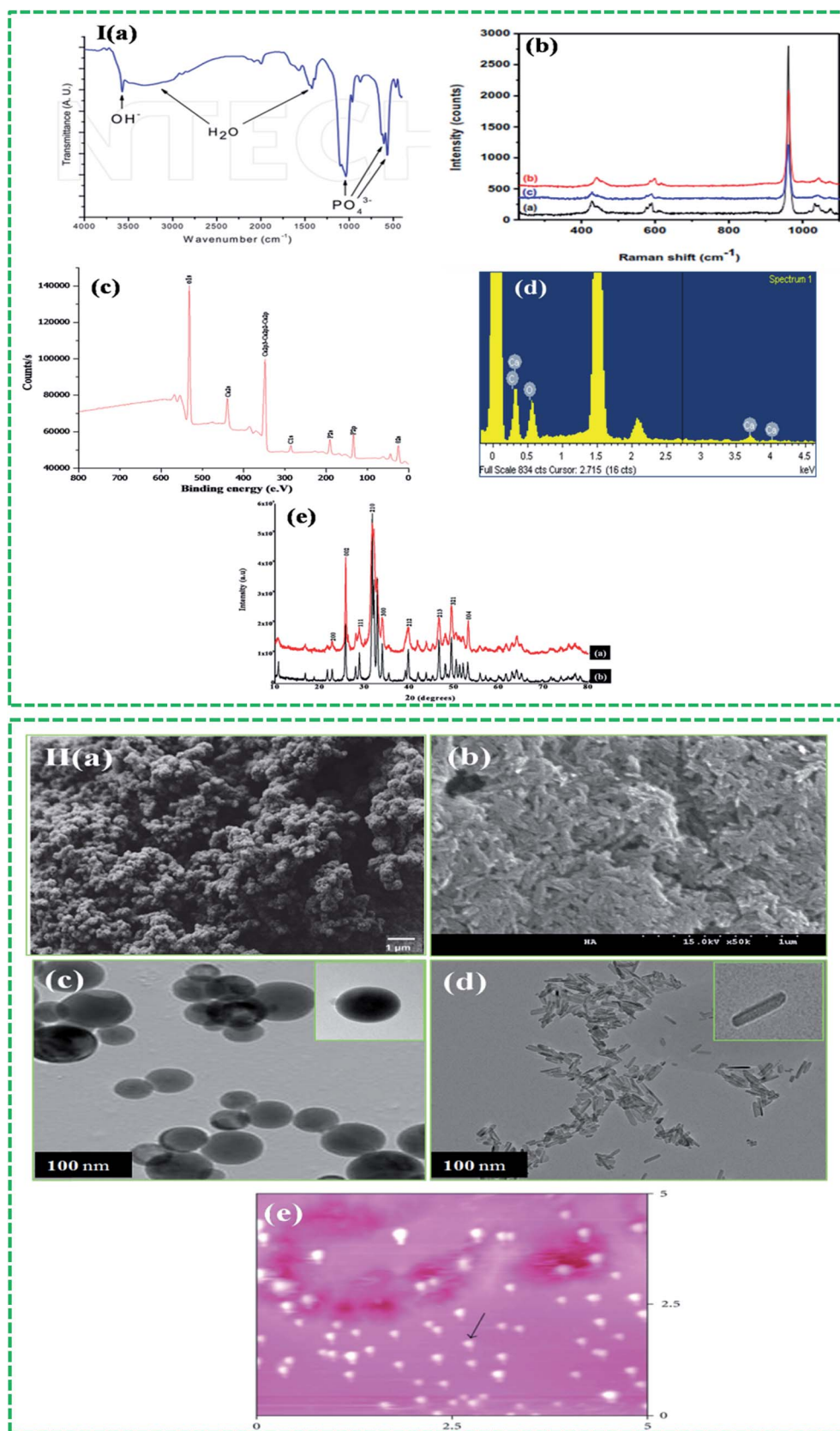
Fig. 5 Techniques used to characterize HA: I (a–e) spectroscopic (reproduced with permission from Springer and INTECH) 10,45,48 and II ((a–e)) ((b) is the unpublished figure owned by authors)) direct visualization (reproduced with permission from Hindawi). 47,49
