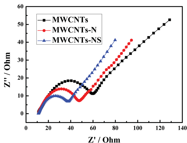
Fig. 4 Electrochemical impedance spectroscopy of glassy carbon electrodes modified by different MWCNTs samples in 1.0 mol L -1 VOSO 4 + 3.0 mol L -1 H 2 SO 4 at open-circuit voltage.
