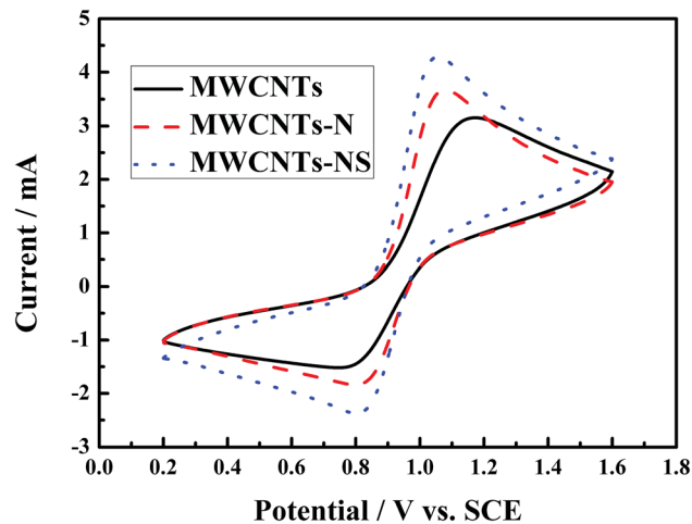
Fig. 3 Cyclic voltammograms of glassy carbon electrodes modified by different MWCNTs samples at the scan rate of 20 mV s -1 in a 2.0 mol L -1 VOSO 4 + 3.0 mol L -1 H 2 SO 4 electrolyte solution.
