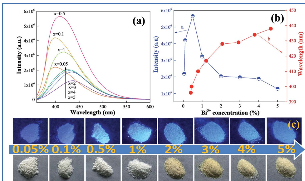
Fig. 3 (a) Emission spectra ( \lambda_{\text{ex}} = 346 nm) of typical samples of CAZO: x\% Bi 3+ ( x = 0.05, 0.1, 0.5, 1, 2, 3, 4 or 5 ). (b) Dependence of the emission intensities on the Bi 3+ concentrations (blue line), and the variation in the red shift of Bi 3+ emission with increasing concentration of Bi 3+ (red line). (c) Photographs of the CAZO: x\% Bi 3+ phosphors with changing the concentration of Bi 3+ under 365 nm UV (upper line) and visible light (lower line).
