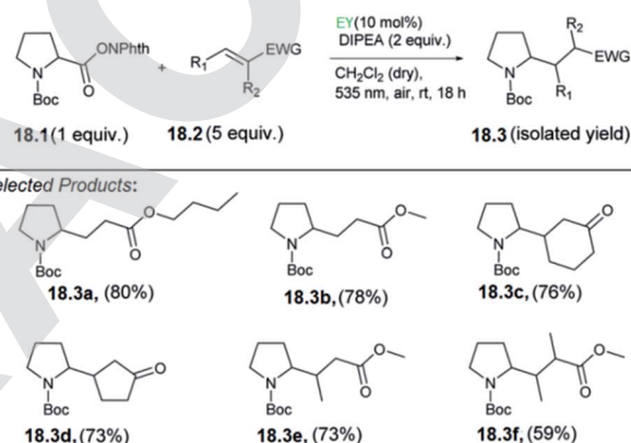
Scheme 18 Decarboxylative alkylation.
