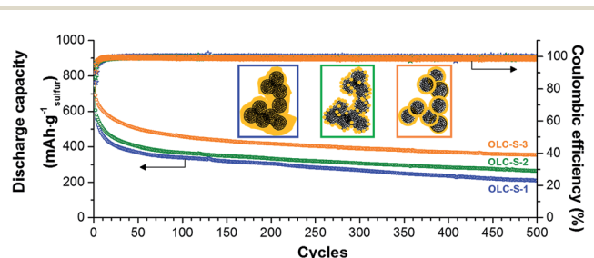
Fig. 6 Long term cycle stability at high C-rates (charging at 2C/discharging at 1C) study of the carbon onion/sulfur hybrids.
