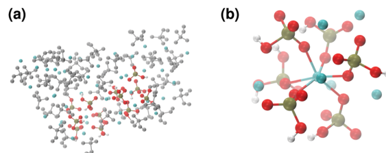
Fig. 5 Solution I: (a) aggregates after 5 ns; (b) detail of one of the Posner-like clusters formed during the simulation with formula [Ca 7 (H 2 PO 4 )(HPO 4 ) 5 ] 3+ . Colour key Ca: light blue, P: green, O: red, atoms not forming Posner's clusters: grey.
