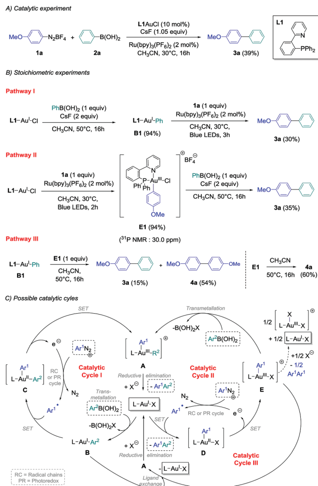
Scheme 2 Catalytic and stoichiometric experiments of the cross-coupling between 4-methoxybenzenediazonium tetrafluoroborate 1a and phenylboronic acid 2a using L1 AuCl as the gold precursor, and possible catalytic cycles.
