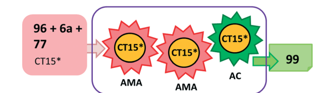
Scheme 29 Tricomponent asymmetric triple cascade reaction catalysed by multi-hollow copolymer microparticles containing immobilized CA6*; AC: aldol condensation. 163
