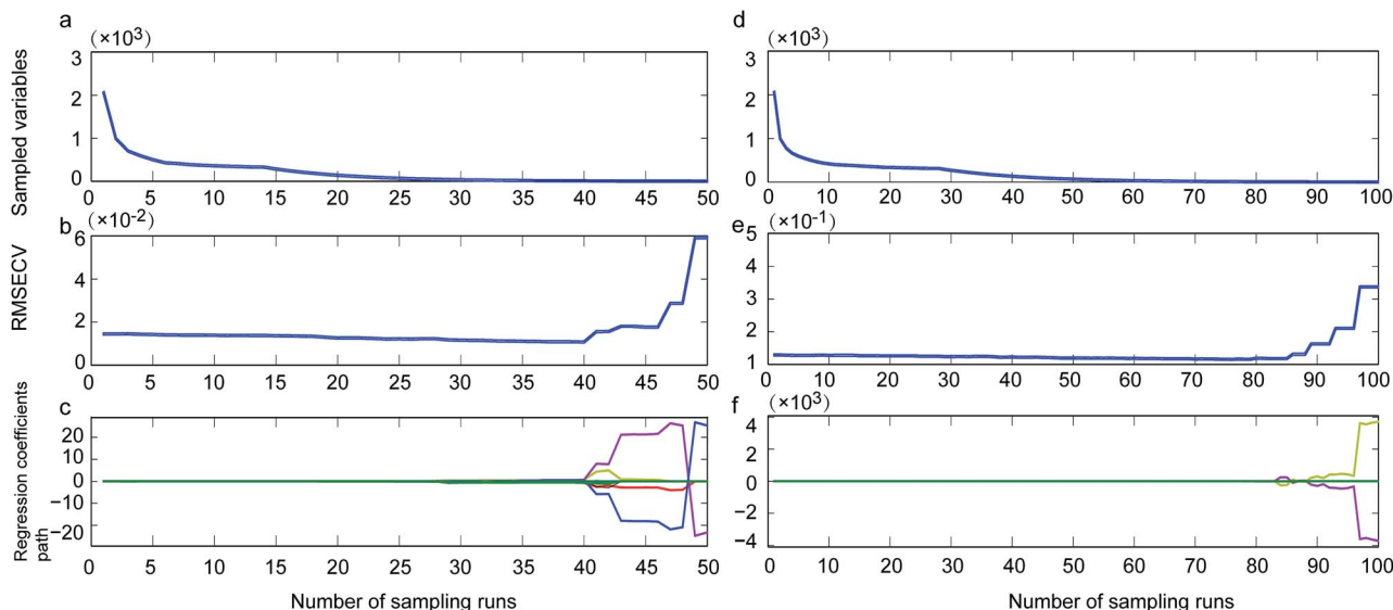
Fig. 4 Changing trend of the sampled wavelength variables (a and d), root mean squared error of cross validation (RMSECV) (b and e) and the regression coefficient path of each variable (c and f) for the single strain recognition model (a–c) and yeast cocktail recognition model (d–f).
