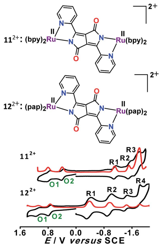
Fig. 12 Cyclic (black) and differential pulse (red) voltammograms in CH_3CN .
