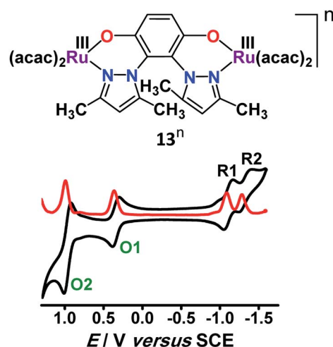
Fig. 14 Cyclic (black) and differential pulse (red) voltammograms of 13 in CH_3CN .
