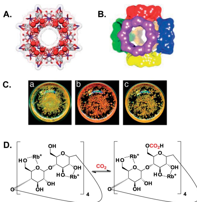
Fig. 2 (A) A ball-and-stick view of a cubic array made of (\gamma\text{-CD})_6 units coordinated to 24\text{ Rb}^+ (red spheres) through the ring oxygen atoms of the secondary and primary hydroxyl groups. (B) A space-filling depiction of six (\gamma\text{-CD})_6 units that link together in a body-centered cubic extended framework. (C) Photographs of CD-MOF-2 incorporating methyl red before (a) and after (b) exposure to \text{CO}_2 . Removal of the \text{CO}_2 atmosphere restored the colour back to yellow (c). A–C are adapted with permission from ref. 41. (D) A proposed carbonation reaction of activated CD-MOF-2 at the less reactive primary hydroxyl groups, where the free hydroxyls act as nucleophiles to attack \text{CO}_2 . 41
