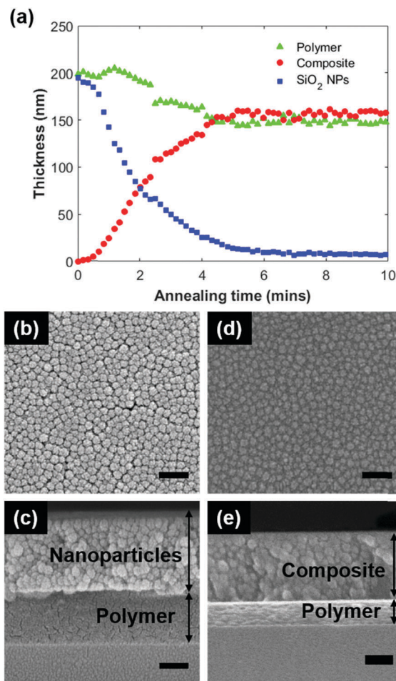
Fig. 2 (a) Thickness profiles of the SiO 2 NP, composite, and neat polymer layers as a function of annealing time, obtained using in situ spectroscopic ellipsometry while annealing \sim 200 nm SiO 2 NP/ \sim 200 nm PS-8k bilayer films at 403 K. The SEM images show the (b) top and (c) cross sectional views of the bilayer film before annealing, and the (d) top and (e) cross sectional views of the PINF atop a residual polymer layer after annealing. The scale bars are 100 nm.
