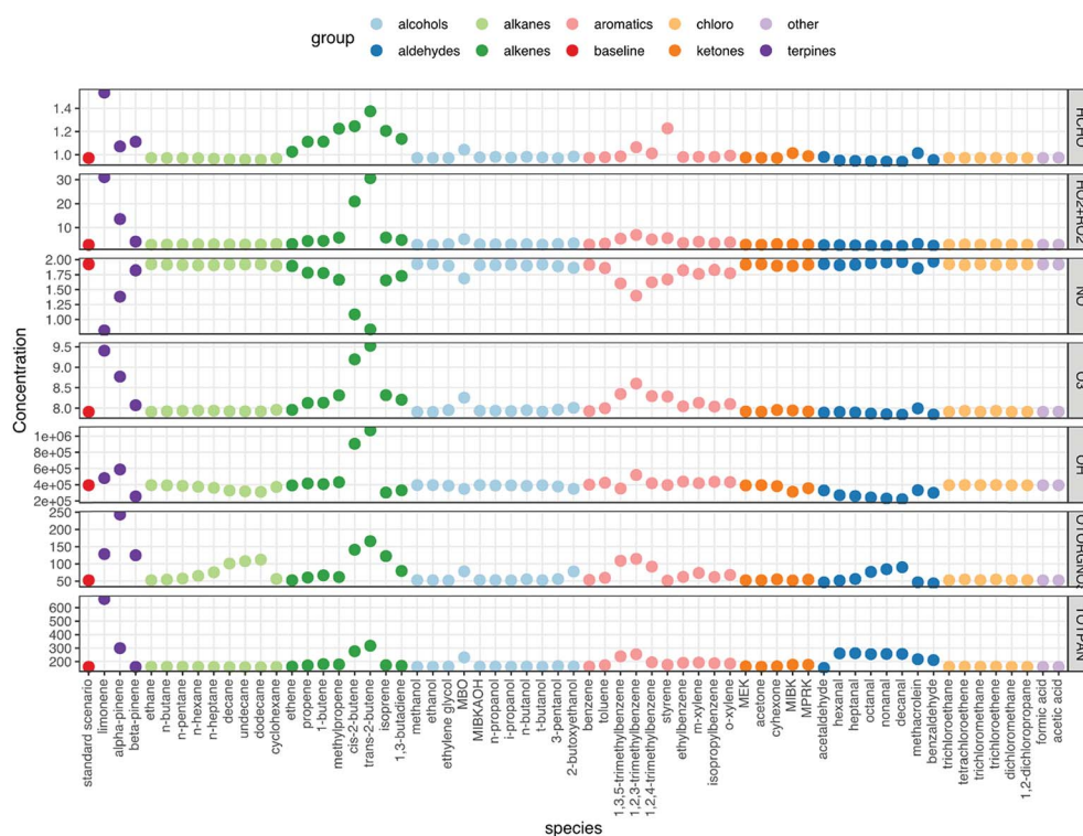
Fig. 2 Changes in mixing ratio for HCHO (ppb), \sum\text{HO}_2 + \text{RO}_2 (ppt), NO (ppb), O 3 (ppb), \sum\text{organic nitrate species} (ppt) and \sum\text{PAN species} (ppt) and concentration of OH (molecule per cm 3 ), with the addition of 10 ppb of different VOCs in turn. The molecules are colour coded according to functionality (see legend) and the standard run (with no VOCs added indoors) is shown in red.
