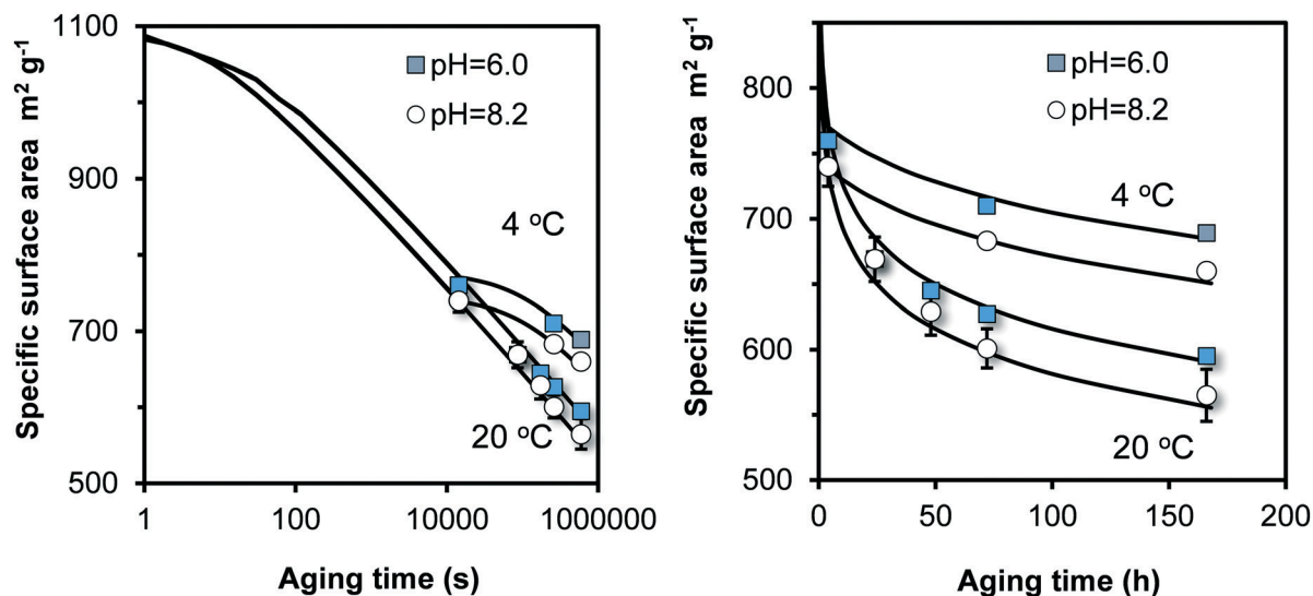
Fig. 6 Time dependency of the specific surface area ( \text{m}^2 \text{g}^{-1} ) for traditionally synthesized Fh, aged in 0.01 M \text{NaNO}_3 in the absence of organic pH buffers. After synthesis at pH 6.0 or 8.2, the Fh materials were aged for 4 hours since neutralization before a first sample was taken. The remaining suspensions were split and further aged at either 4 °C or 20 °C. The lines have been calculated with the model (eqn (8)), only adjusting the rate constant k . At 20 °C, \log k = 9.25 (pH = 8.2) and 9.00 (pH = 6), and at 4 °C, \log k = 8.35 (pH = 8.2) and 8.10 (pH = 6) with k in Fe per \text{m}^2 per second. Subtracting a value of 14.22 from these \log k values gives \log k in the unit \mu\text{mol m}^{-2} \text{s}^{-1} .
