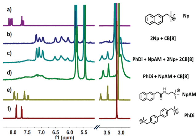
Fig. 2 Partial ^1\text{H} NMR spectra ( 400\text{ MHz} , \text{D}_2\text{O} , 25.0\text{ }^{\circ}\text{C} ) of (a) Np ( 2.0\text{ mM} ); (b) 2Np-CB[8] ( 1.0\text{ mM} ); (c) a mixture of Np ( 2.0\text{ mM} ), NpAM ( 1.0\text{ mM} ), PhDi ( 1.0\text{ mM} ), and CB[8] ( 2.0\text{ mM} ); (d) PhDi-NpAM-CB[8] ( 1.0\text{ mM} ); (e) NpAM ( 1.0\text{ mM} ); (f) PhDi ( 1.0\text{ mM} ).
