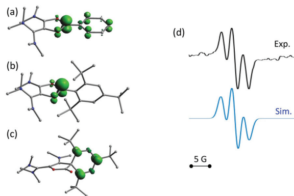
Fig. 4 Representation of computed Mulliken spin densities for, (a) 6a , (b) 6d and (c) 11d ; (d) experimental X-band isotropic EPR spectrum at room temperature in acetonitrile after reduction of 6d (top, in black), the simulated spectrum (bottom, in blue) was obtained with a Lorentzian line-broadening parameter of 0.25 and an hyperfine constant a(^1\text{H}) of 8.0 MHz (2 nuclei).
