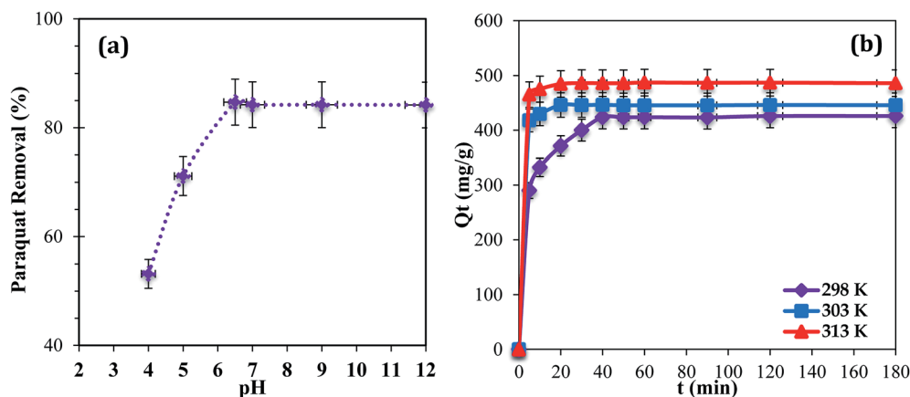
Fig. 4 (a) Effect of initial solution pH ( T = 298\text{ K} ; C_i = 100\text{ mg L}^{-1} ; m = 20\text{ mg} ). (b) Effect of contact time (temperature: 298, 303, and 313 K; C_i = 100\text{ mg L}^{-1} ; m = 20\text{ mg} ; pH = 6.5).
