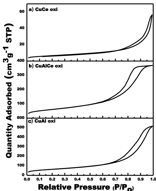
Fig. 1 Adsorption/desorption isotherms for calcined Cu supported catalyst: CuCe oxide, CuAlCe oxide and CuAl oxide.
