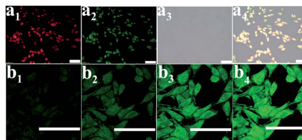
Fig. 5 Fluorescence images of HeLa cells (a) red channel indicating PCNH fluorescence ( a_1 ), green channel corresponding to DCFH-DA ( a_2 ), bright field ( a_3 ) and the merged image ( a_4 ). (b) ROS cumulative production photographs taken by a confocal laser scanning microscope with DCFH-DA as the indicator (excitation interval is 2 min).
