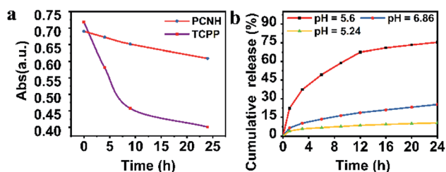
Fig. 4 Photostabilities of PCNH and TCPP when exposed to natural light for 24 h (a). Cumulative release of TCPP from PCNH in different pH solutions (b); the concentration of PCNH is 1 \text{mg mL}^{-1} .
