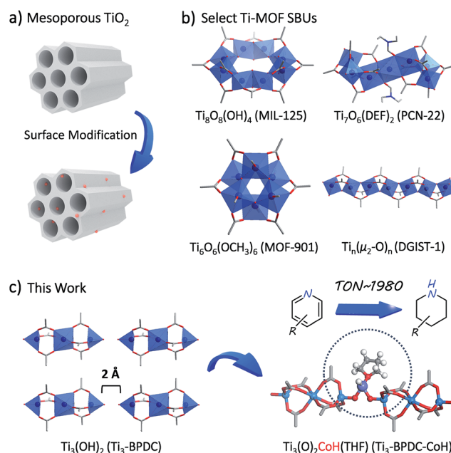
Fig. 1 (a) Surface modification of mesoporous TiO_2 generates functional materials. (b) Select Ti-MOF SBU structures (MIL-125, PCN-22, MOF-901, and DGIST-1). (c) Schematic illustration of novel Ti_3(OH)_2 SBUs in Ti_3 -BPDC and their metalation to generate anchored Co^{II} -H species for cascade reduction of N-heteroarenes.
