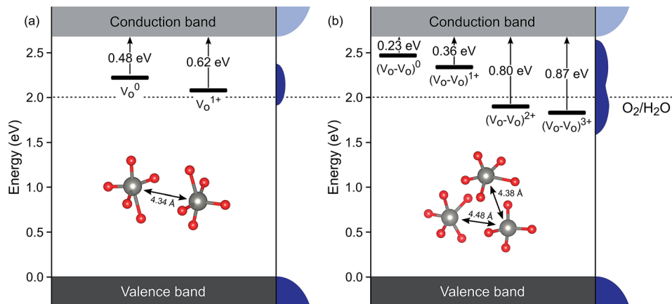
Fig. 3 Defect ionisation levels of oxygen vacancies in different charge states calculated from hybrid density functional theory for (a) an isolated oxygen vacancy V_{\text{O}}^{\text{y}} and (b) a defect complex composed of two oxygen vacancies V_{\text{O}}^{\text{z}} . Energies are relative to the valence band edge. Densities of states are illustrated schematically at the right side of each panel. The insets show local atomic structures and the distance between the W atoms.
