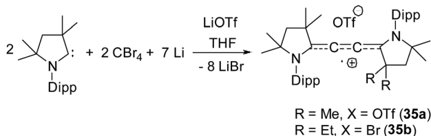
Fig. 8 Synthesis of di-cAAC stabilized C_2^{+} .
