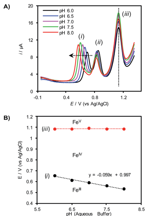
Fig. 2 (A) Differential pulse voltammograms of 0.5 mM 1 in 1 : 1 \text{CH}_3\text{CN} : \text{buffer} (0.1 M phosphate). (B) Pourbaix diagram derived from the peak potentials of redox features (i) and (iii) in (A).
