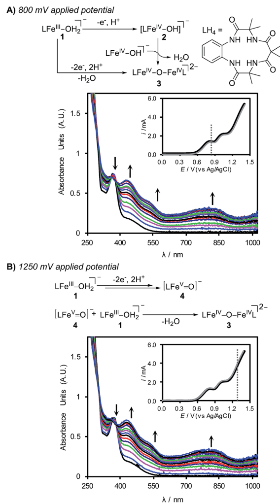
Fig. 3 (A) UV-vis spectra recorded for 0.5 mM 1 undergoing bulk electrochemical oxidation at 800 mV (vs. Ag/AgCl) in 1 : 1 \text{CH}_3\text{CN} : \text{H}_2\text{O} with \text{K}_2\text{HPO}_4 (0.1 M) in a divided cell. Final spectra collected after 15.3 min of bulk electrolysis. (B) UV-vis spectra recorded for 0.5 mM (TAML)Fe undergoing bulk electrochemical oxidation at 1250 mV (vs. Ag/AgCl) in 1 : 1 \text{CH}_3\text{CN} : \text{H}_2\text{O} with \text{K}_2\text{HPO}_4 (0.1 M) in a divided cell at a RVC electrode. Final spectra collected after 6.7 min of bulk electrolysis. (Inset) LSV of bulk electrolysis solution at the RVC working electrode. The potential applied for each bulk electrolysis is indicated. Continuing electrochemical oxidation beyond the final spectra shown in (B) leads first to steady state absorption features followed by overall loss of all (TAML)Fe absorption features.
