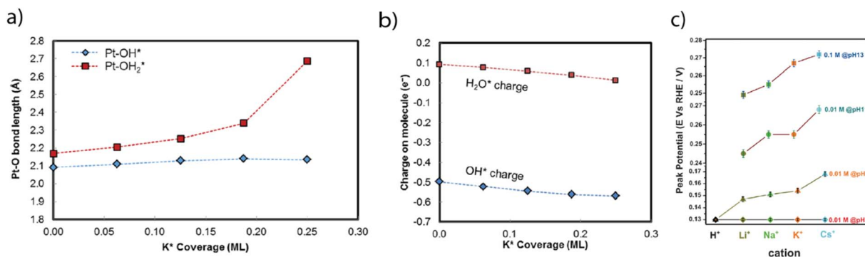
Fig. 6 (a) Pt–O bond lengths and (b) Bader charge for adsorbed OH and H_2O molecules on Pt(100) calculated using DFT at different adsorbed potassium coverages (reproduced from ref. 16 with permission from the American Chemical Society, Copyright (2016)), and (c) experimental position of the OH_{ad}/H^* peak on Pt(533)_{ad} at different pH values with different alkali cation contents (reproduced from ref. 17 with permission from John Wiley and Sons, Copyright (2017)).
