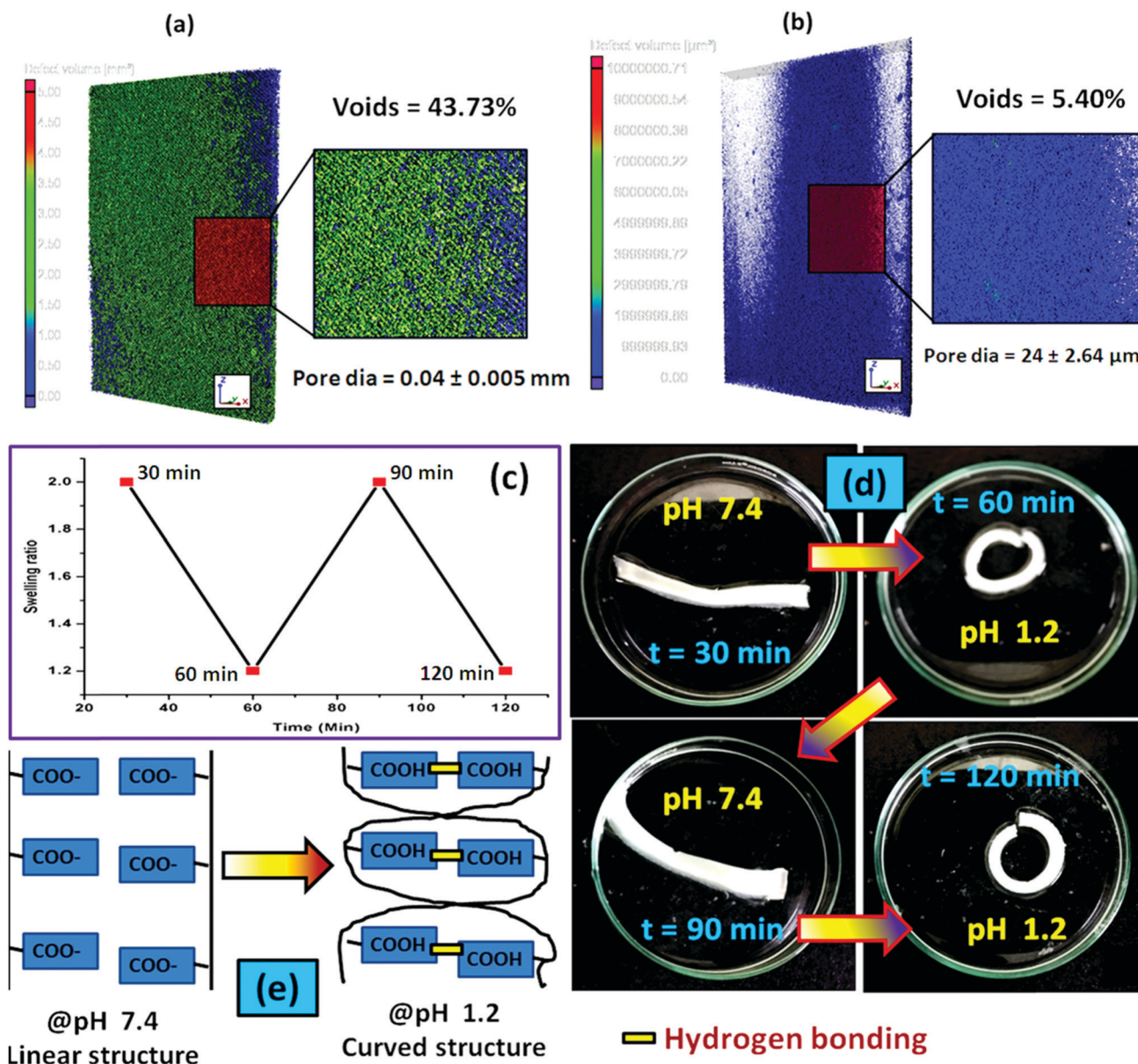
Fig. 8 Micro CT analysis of the hydrogel having a composition of (a) PSAS 0 C 0 and (b) PSAS 50 C 5 ; (c) actuation cycle of the composite hydrogel (PSAS 50 C 5 ) in the presence of acid (pH 1.2); (d) acid induced actuation in the composite hydrogel system (PSAS 50 C 5 ) and (e) probable mechanism lying behind the actuation.
