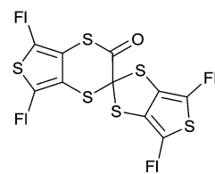
Fl = fluorene or oligofluorene
