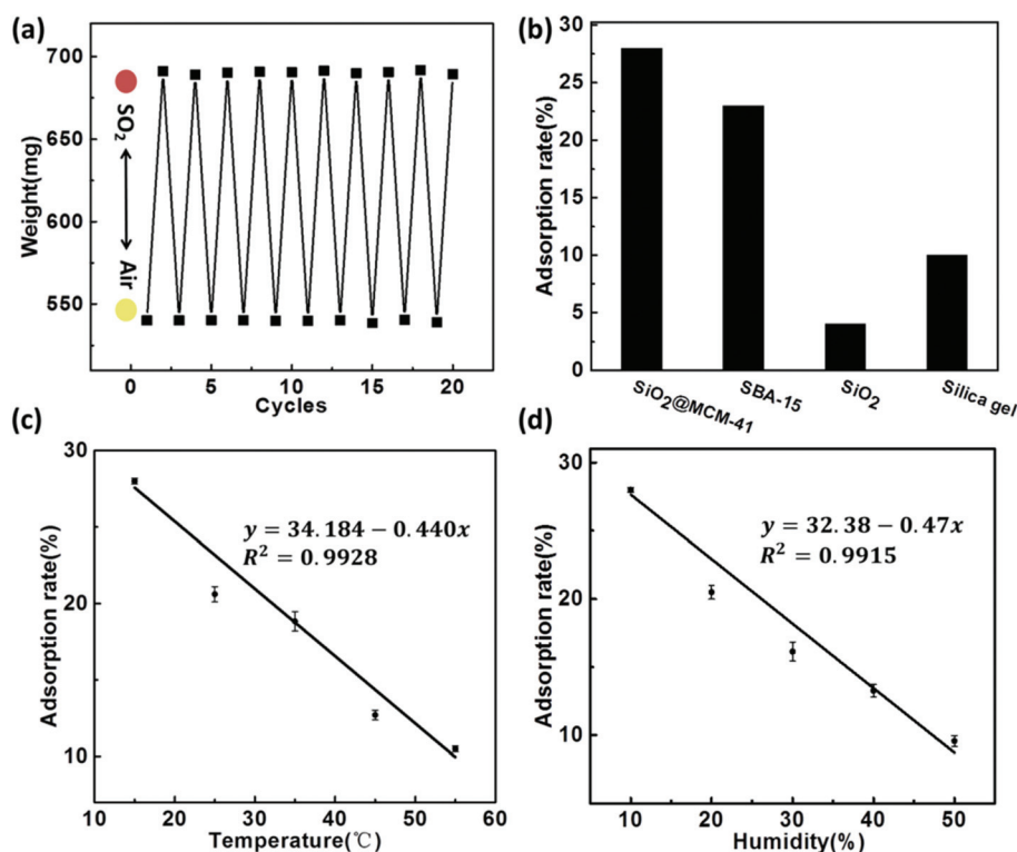
Fig. 3 (a) Reversible changes of the weight of \text{SiO}_2@MCM-41 when alternately exposed to air and \text{SO}_2 gas, and the corresponding color changes. (b) The adsorption rates of \text{SiO}_2@MCM-41 , SBA-15, silica gel and \text{SiO}_2 toward \text{SO}_2 gas. (c) The relationship between the adsorption rate and the temperature of \text{SO}_2 gas. (d) The relationship between the adsorption rate and the humidity of \text{SO}_2 gas.
